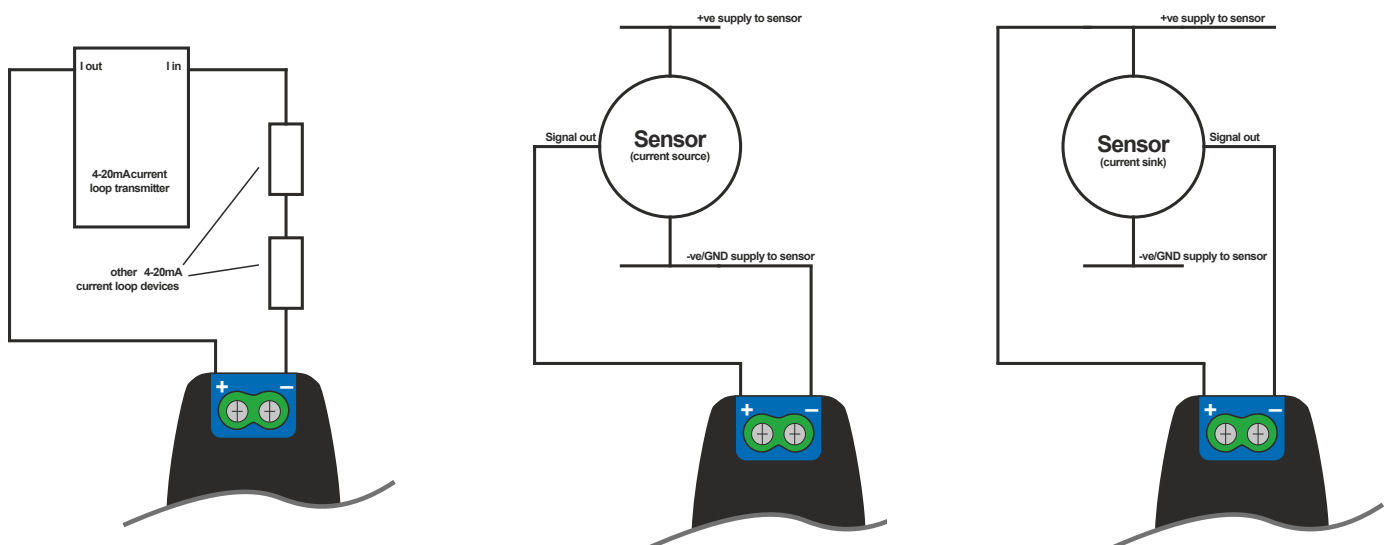
Connecting to a current loop transmitter.
