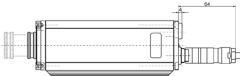
Pyrometer with thru-lens view finder
